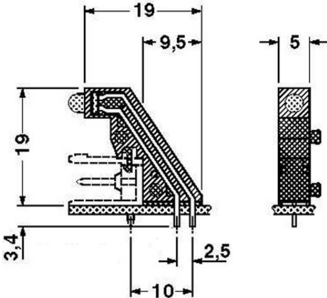
Dimensional drawing
